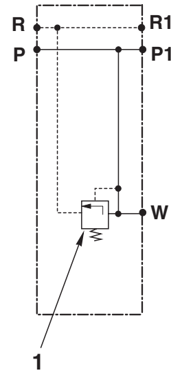
SCHEMA HYDRAULIQUE
